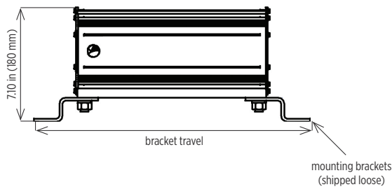
Side View: Bracket Mounting
