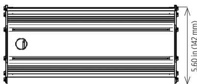
Assembled Top View
