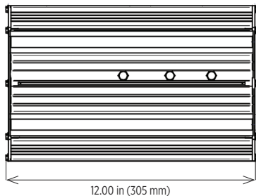
Assembled Front View
