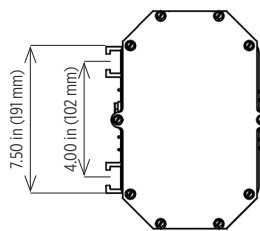
Assembled Side View
