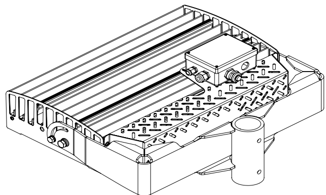
CF-250 NPL Bracket
