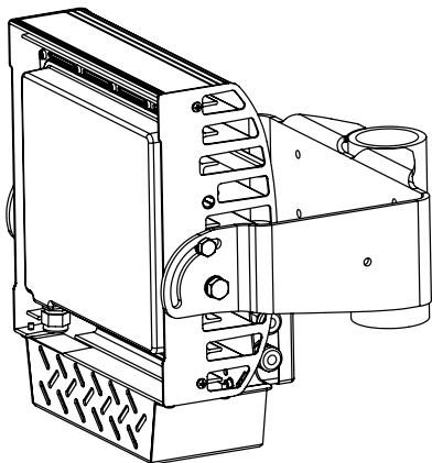
CF-150 NPL Bracket
